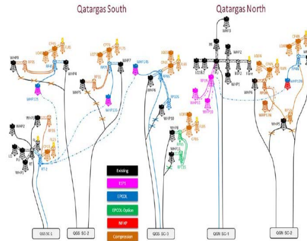
Figure 1: Schematic for the North Field Production Sustainability Offshore & Pipelines Project
