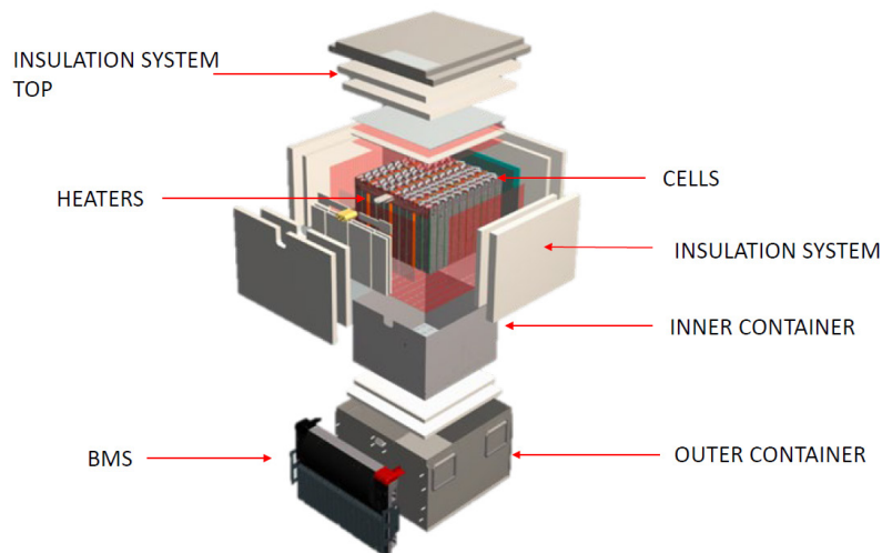
SMC Battery Module Contents
